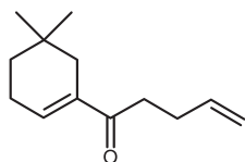
1-(5,5-dimethyl-1-cyclohexen-1-yl) -4-penten-1-one
